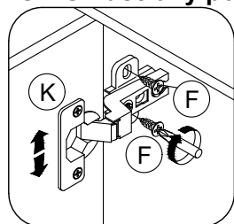
Vertical Adjustment
