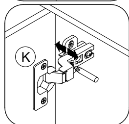
Depth Adjustment
